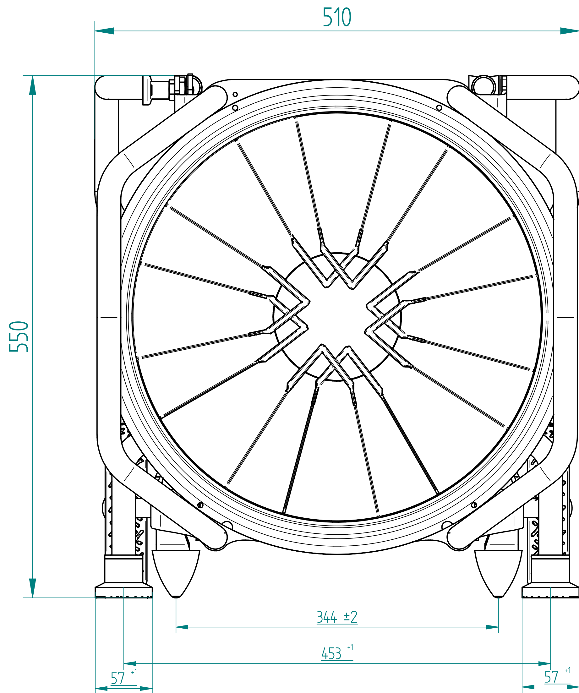
Front View
